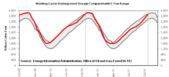
Above Graph - Storage levels as of 10-27-11
